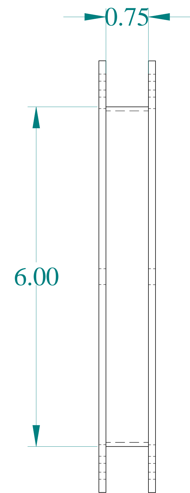
FRONT VIEW
