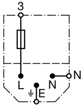
with internal connections 1-pole
