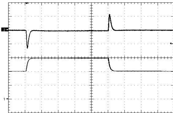
Figure 15. Load Transient Response (50mV/div), di/dt=0.1A/\mu S , 50% - 75% - 50% of full load, C_{out}=Fig3 time scale: 200µS/div. Ch1=Vout, Ch2=Iout (1A/div)
