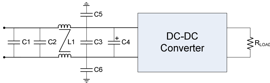
Figure 22. EMI Filter
