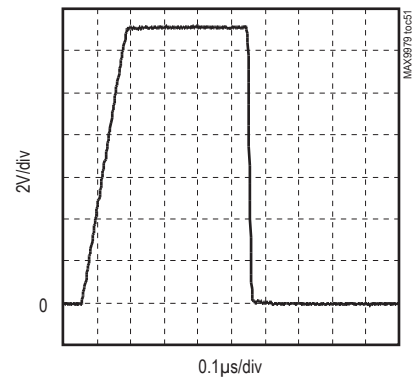
TRANSIENT RESPONSE VHH
