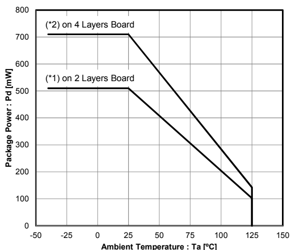
NJW4615AF1 (SOT-23-6) Power Dissipation (Topr=-40°C to +125°C, Tj=150°C)
