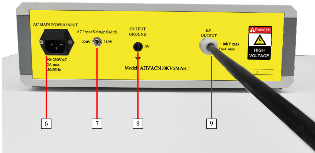
Figure 3. Back Panel
