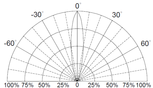
Fig.6 Directive Radiation
