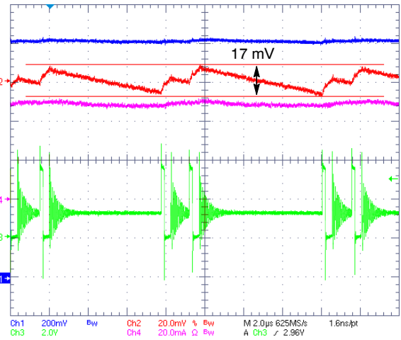
Figure 25. PFM Ripple
