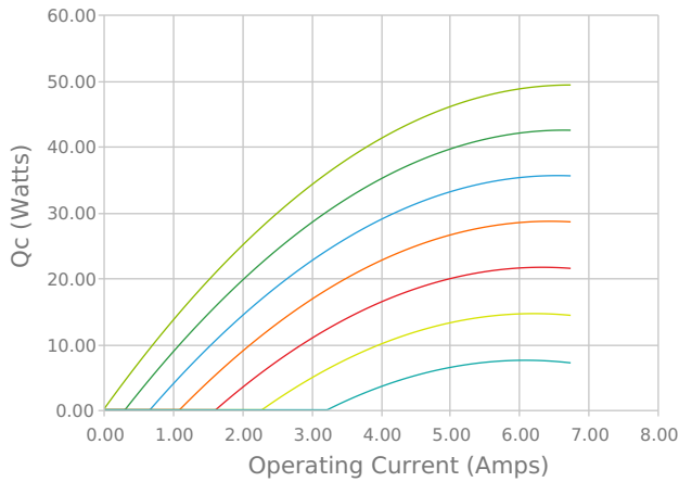
Heat Pumped at Cold Side That = 27 °C
