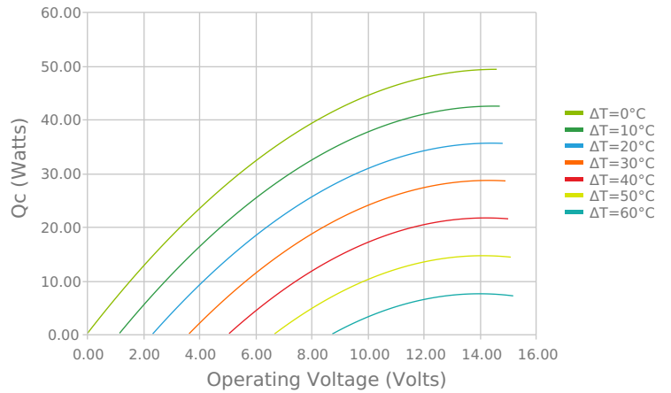
Heat Pumped at Cold Side That = 27 °C
