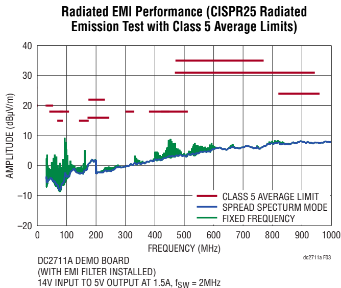
Figure 3. LT8608S Demo Circuit EMI Performance in CISPR25 Radiated Emission Test, Antenna Polarization: Horizontal ( V_{IN} = 14\text{V} , V_{OUT} = 5\text{V} , I_{OUT} = 1.5\text{A} , 2MHz Switching Frequency)
