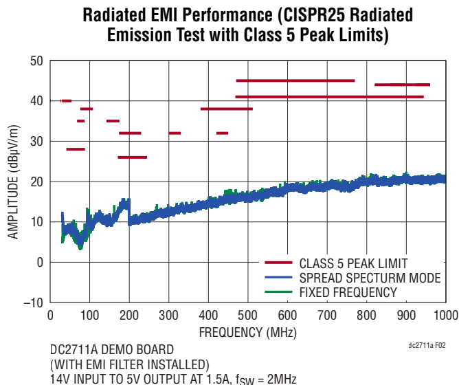
Figure 2. LT8608S Demo Circuit EMI Performance in CISPR25 Radiated Emission Test, Antenna Polarization: Vertical ( V_{IN} = 14\text{V} , V_{OUT} = 5\text{V} , I_{OUT} = 1.5\text{A} , 2MHz Switching Frequency)
