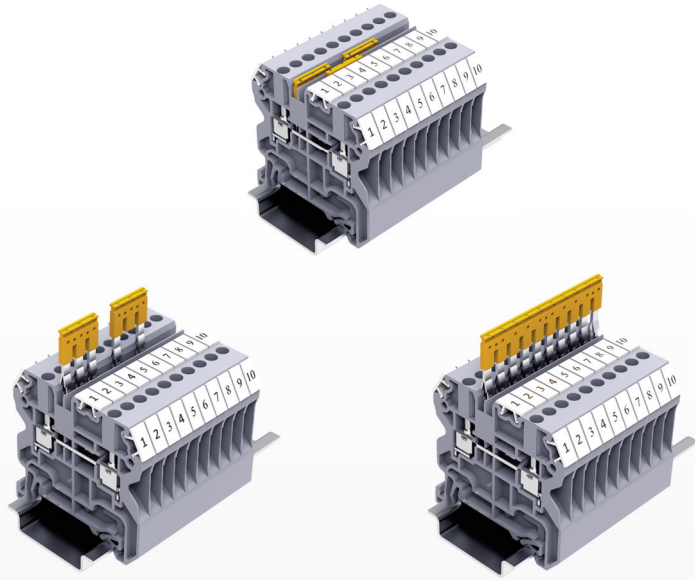
2 Jumper Channels
