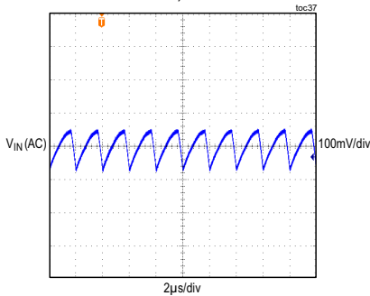
MAXM15062 INPUT VOLTAGE RIPPLE V_{IN} = 24V , FIXED V_{OUT} = 3.3V , FULL LOAD, PWM MODE
