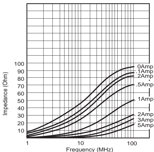
IMPEDANCE VS. DC BIAS SMB30 & SMB40
