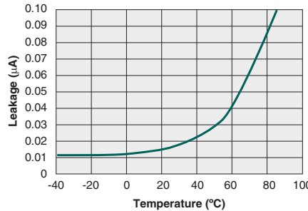
Typical Leakage vs. Temperature Measured across Pins 15&16
