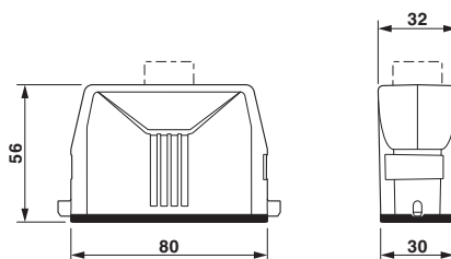
Dimensional drawing
