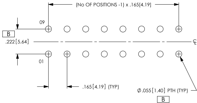
FIG 1 DOUBLE ROW LAYOUT SHOWN FOR IPBS-108-X1-X-D
