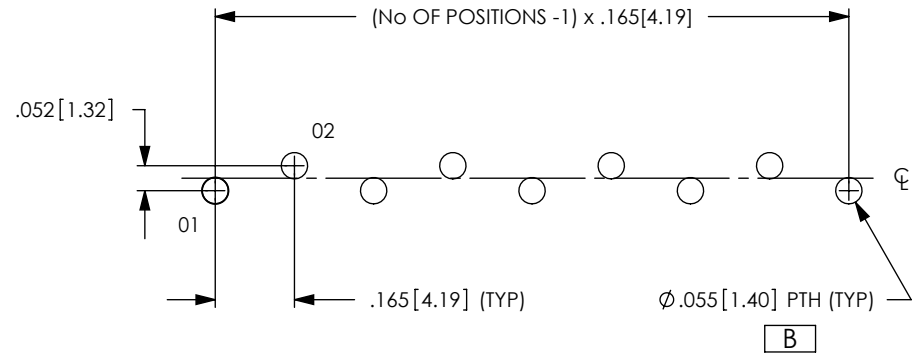
FIG 2 SINGLE ROW * NOT RELEASED FOR PRODUCTION (LAYOUT SHOWN FOR IPBS-109-X1-X-S)
