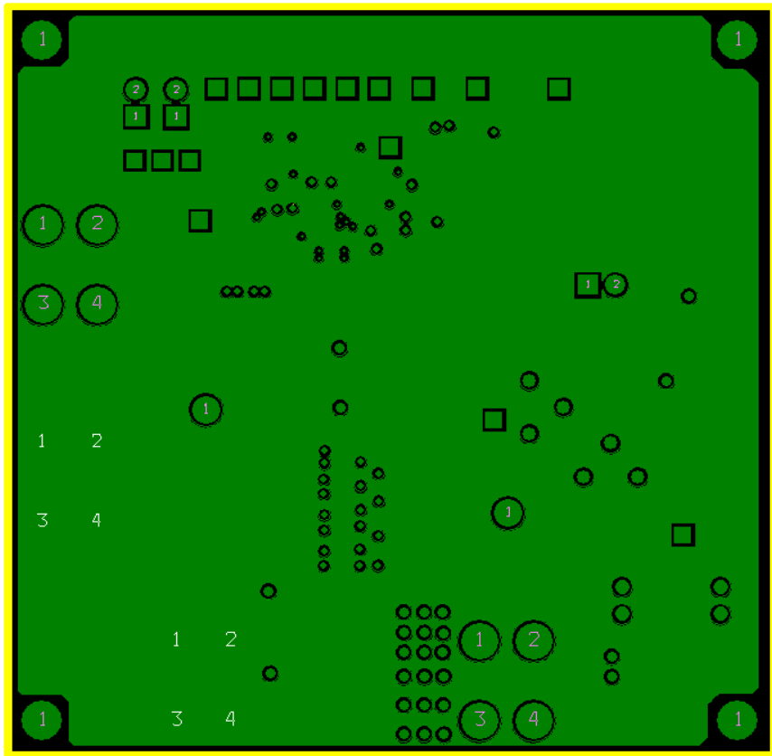
Figure 25. Evaluation Board Inner Layer 2 Copper
