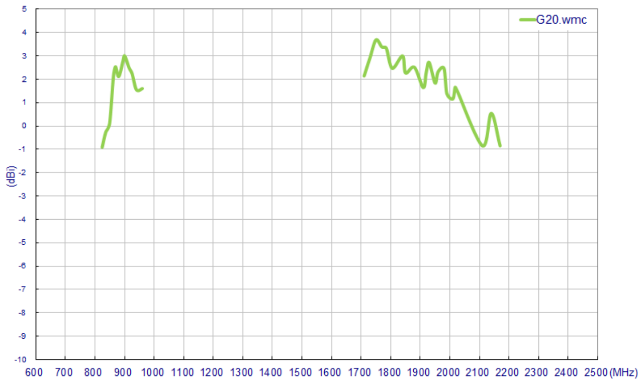
Figure4. Peak gain of G20.B.305111.wmc with 3 meters cable length
