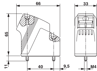
Dimensioned drawing
