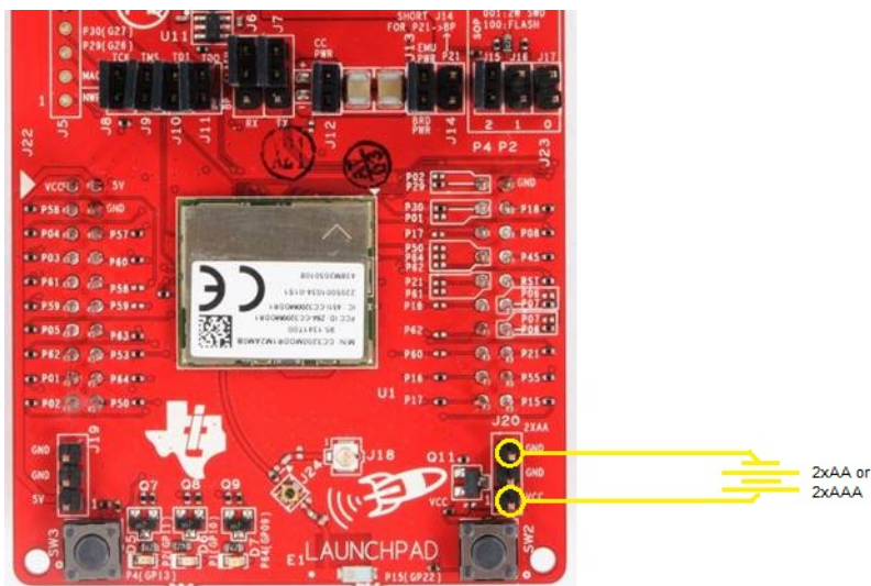
Figure 10. Battery Power
