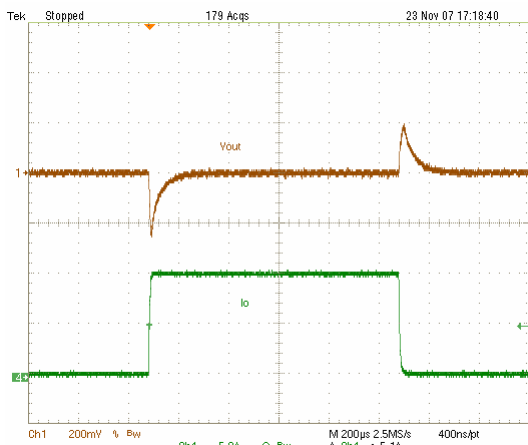
Fig. 8 Transient Response
