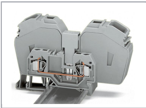
Commoning with step-down jumper (283-414) from
