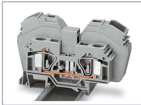
The following 285 Series Through Terminal Blocks can be commoned with 283 Series Through Terminal Blocks:
