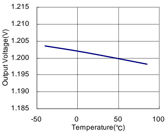
RP501K121x(PWM fixed)
