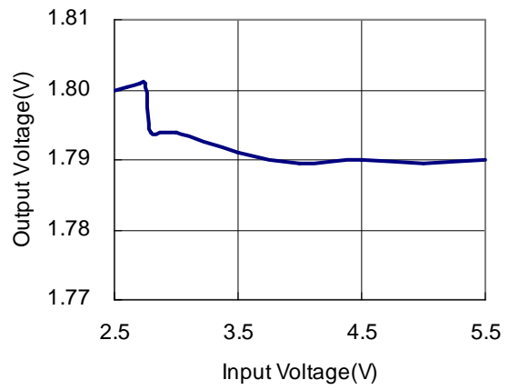
RP501K181x(PWM/VFM modechange) MODE=VIN ,I OUT =1mA
