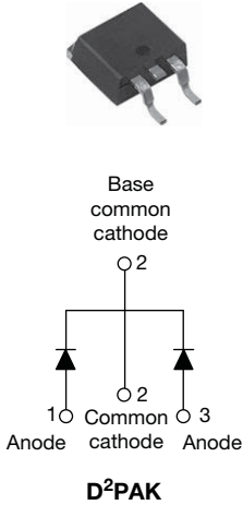
VS-15CTQ...SPbF
