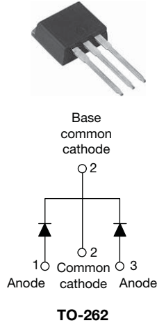
VS-15CTQ...-1PbF
