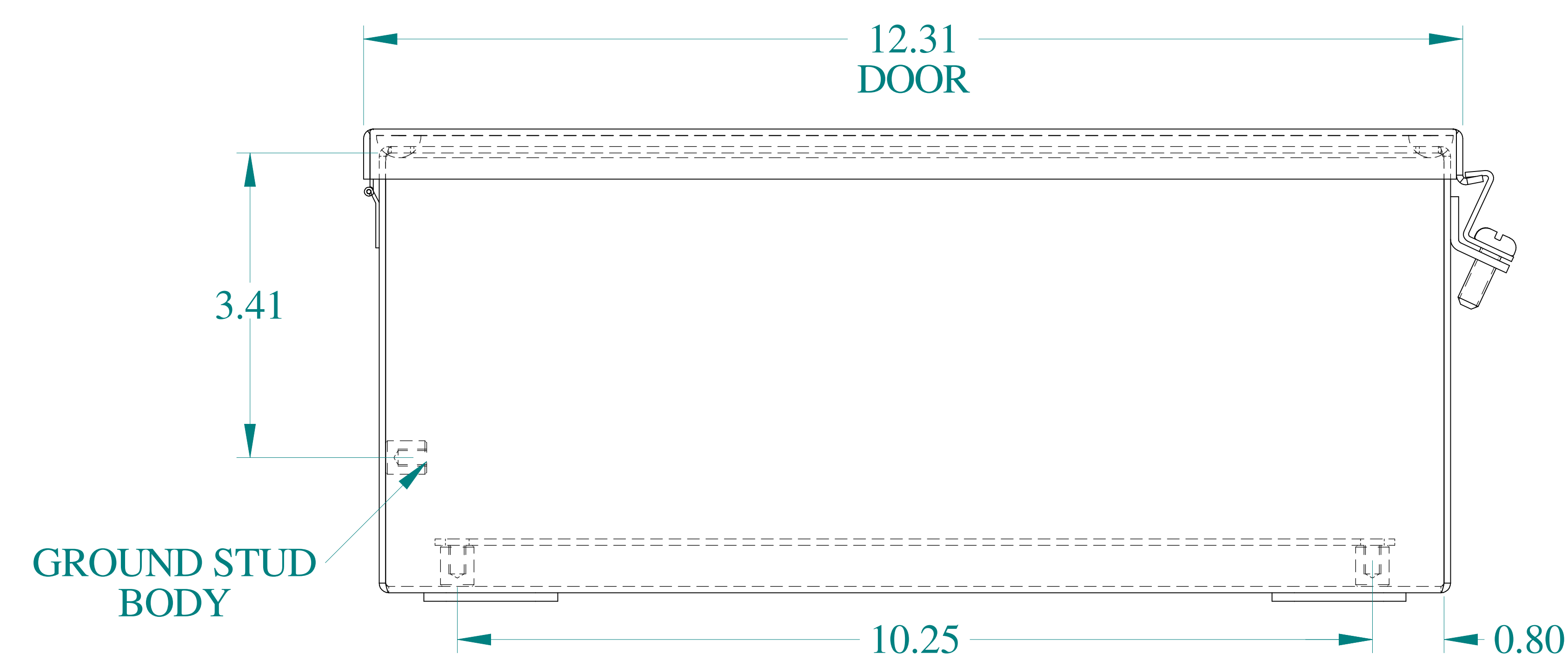
BOTTOM VIEW
