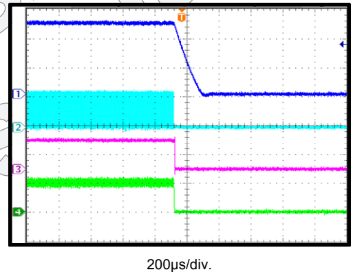
ENPWR Bit Disable through I2C Command , Load=5A
