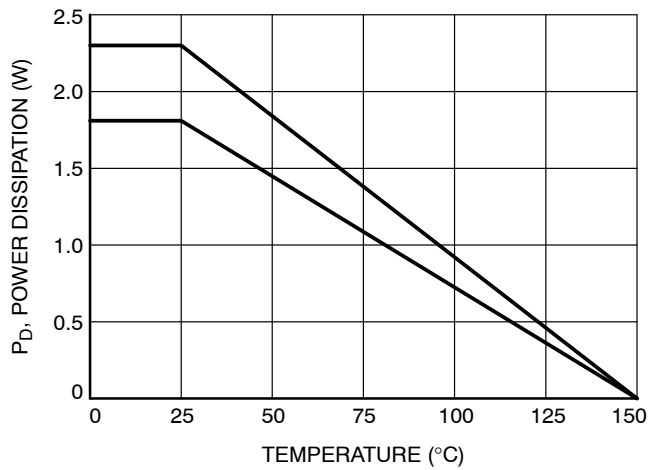
Figure 12. Power Derating
