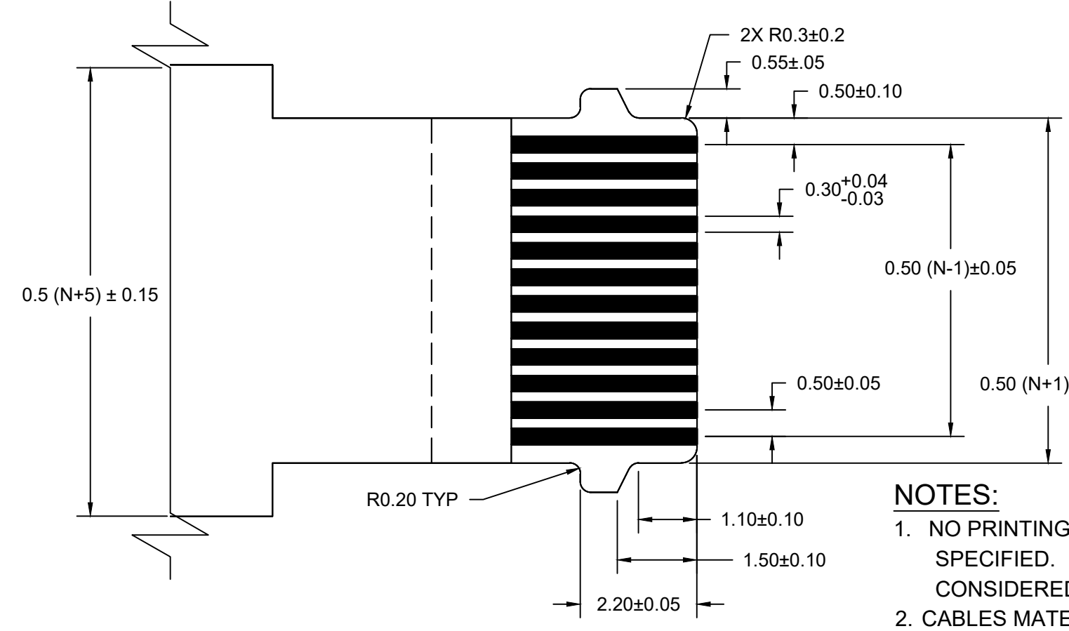
END-TAIL DIMENSIONS SCALE 10:1
