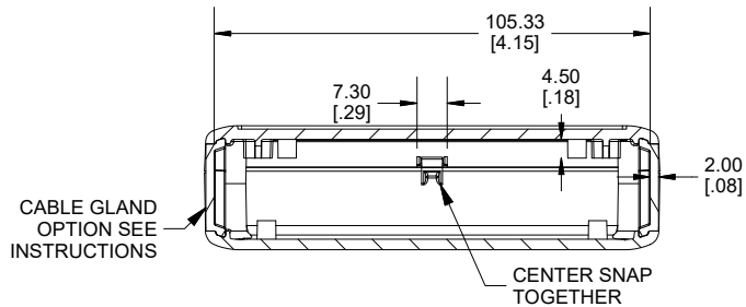
SECTION A-A SIDE VIEW
