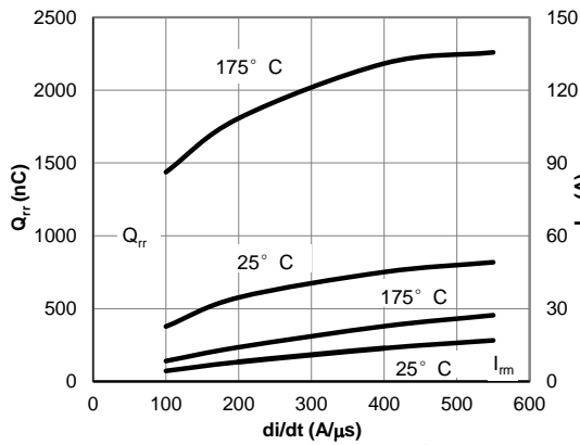
Figure 7: Diode Reverse Recovery Charge and Peak Current vs. di/dt ( V_{GE}=15V, V_{CE}=400V, I_F=40A )
