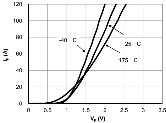
Figure 1: Diode Characteristic
