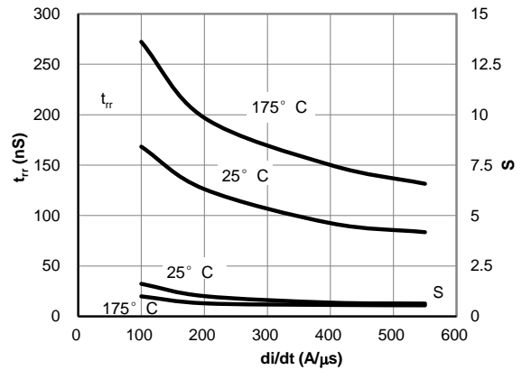
Figure 8: Diode Reverse Recovery Time and Softness Factor vs. di/dt ( V_{GE}=15V, V_{CE}=400V, I_F=40A )
