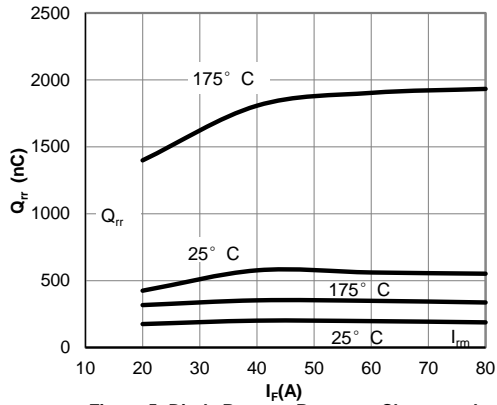
Figure 5: Diode Reverse Recovery Charge and Peak Current vs. Conduction Current ( V_{GE}=15V, V_{CE}=400V, di/dt=200A/\mu s )
