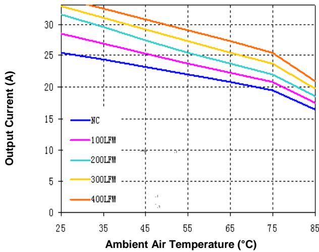
Figure 9. Current Derating Curve for Airflow Direction 3 (Ref. Fig. 10 for Airflow Direction; typical V_{in} , open frame)
