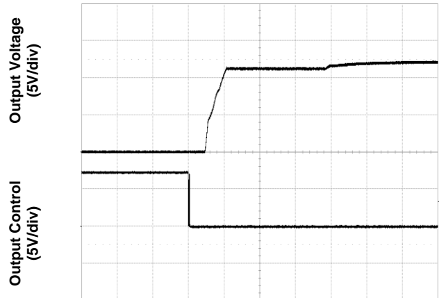
Figure 6. Start-Up from Enable Control (typical Vin, zero load)
