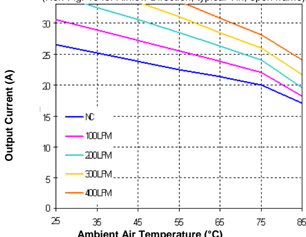
Figure 11. Current Derating Curve With Baseplate
