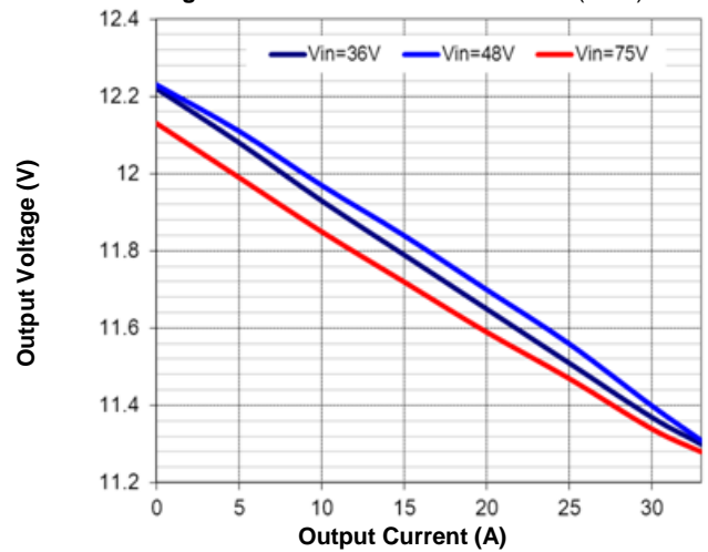
Figure 4. Output Characteristics (parallel version)
