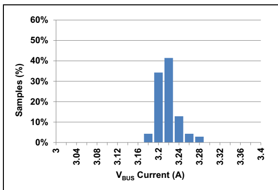
FIGURE 2-20: ILIM8 Trip Current Distribution.
