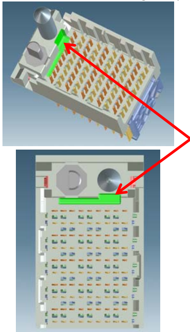
Before – notch next to the guide pin
