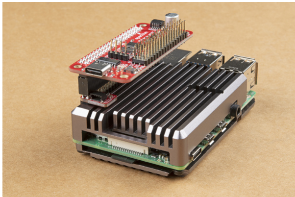
Extension Header with 9.80mm Pin Length is Used to Help Stack the Qwiic SHIM and Pi Servo HAT on a Pi 4 with Heat Sink
