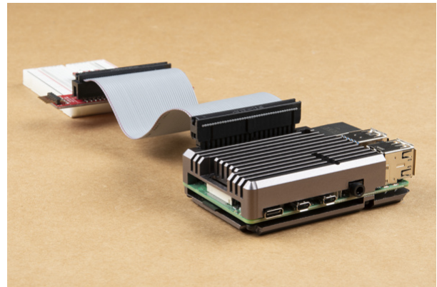
Extension Header with 7.30mm Pin Length is Used to Help Connect the Pi Wedge's IDC Cable to the Pi 4 with Heat Sink
