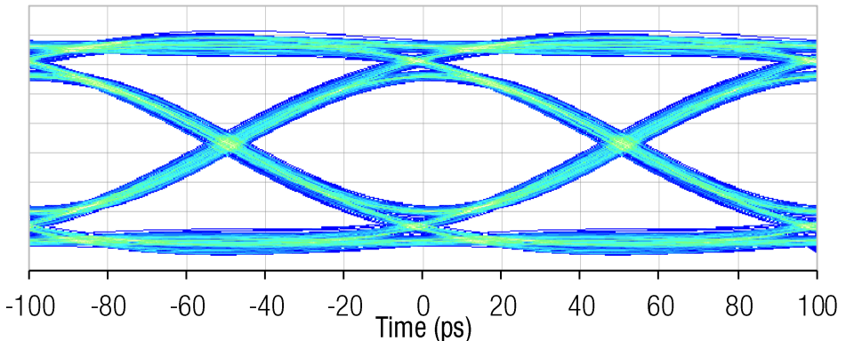
Eye diagram of the dongle with activated USB equalizer (@ 10 GBit/s).
