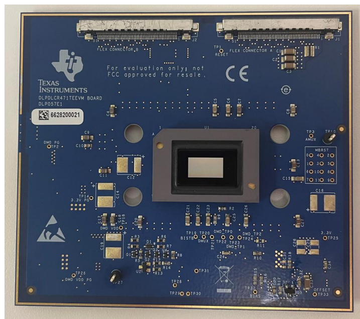
Figure 1-3. DLP471TEEV
