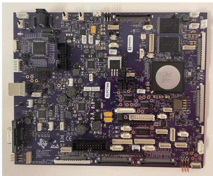
Figure 1-1. DLPC7540EVM Formatter Board
