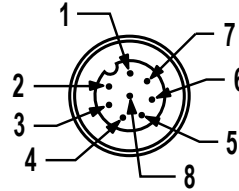
Euro-style Male Pinouts
