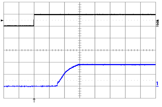
Figure 18. Turn-on transient at full rated load current (resistive) plus 10,000 \mu\text{F} at V_{in} = 48\text{ V} , triggered via ON/OFF pin. Top trace: ON/OFF signal (5 V/div.). Bottom trace: output voltage (1 V/div.). Time scale: 1 ms/div.
