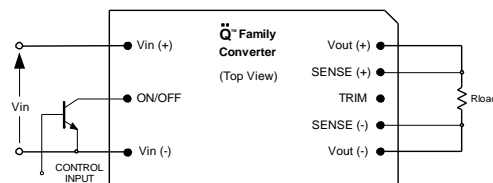
Figure 1. Circuit configuration for ON/OFF function.
