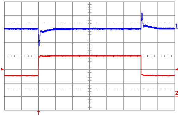
Figure 20. Output voltage response to load current step-change (7.5 A – 15 A – 7.5 A) at V_{in} = 48 V. Top trace: output voltage (100 mV/div.). Bottom trace: load current (5 A/div.). Current slew rate: 5 A/ \mu s. C_o = 450 \mu F tantalum + 1 \mu F ceramic. Time scale: 0.2 ms/d
