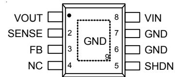
RT9068 SOP-8
