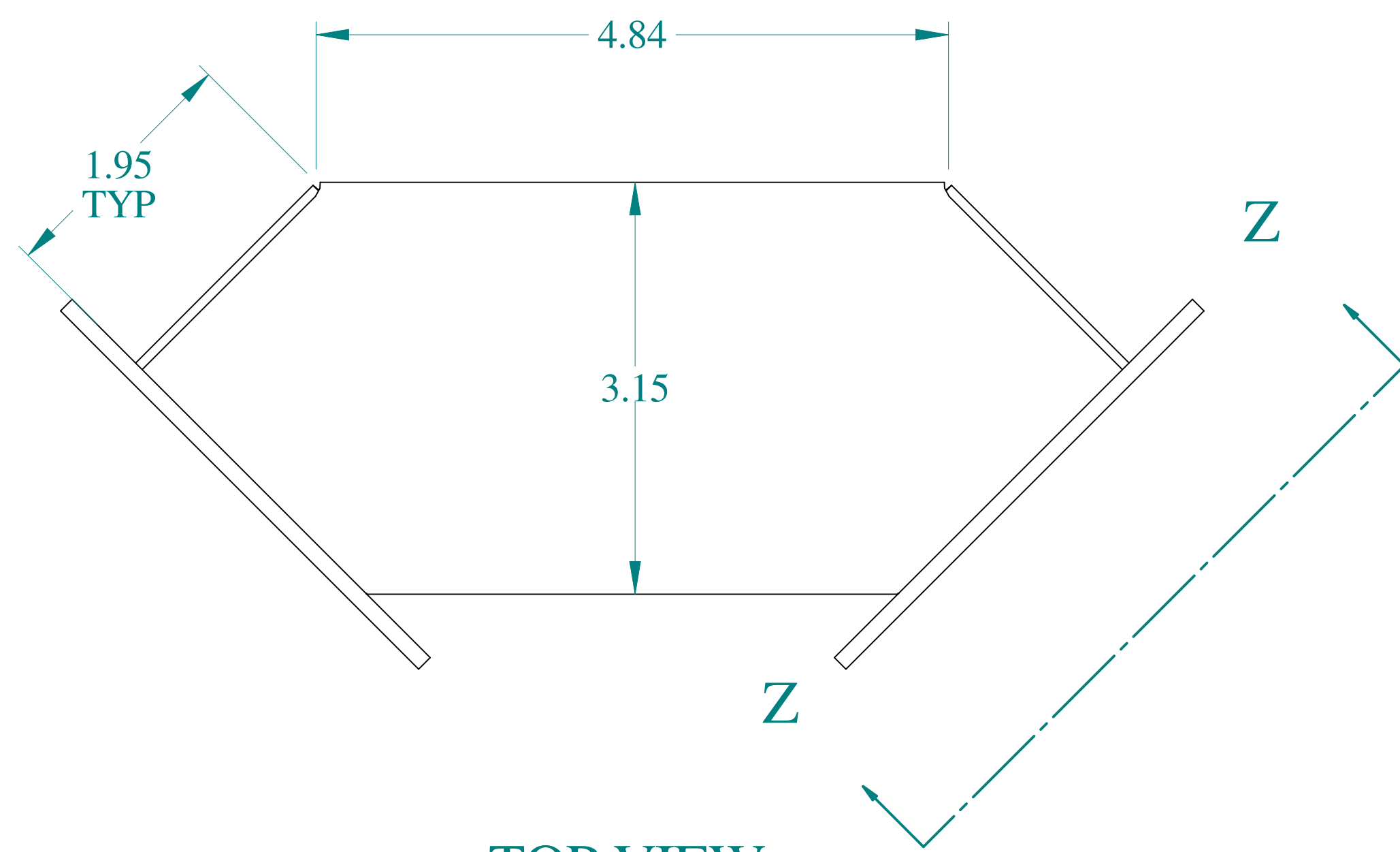
TOP VIEW
