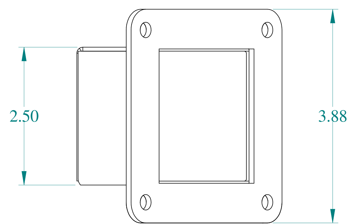
SIDE VIEW
