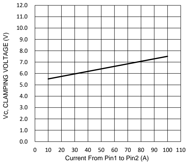
Figure 5 Clamping Voltage Characteristic ( t_p=8/20\mu s )
