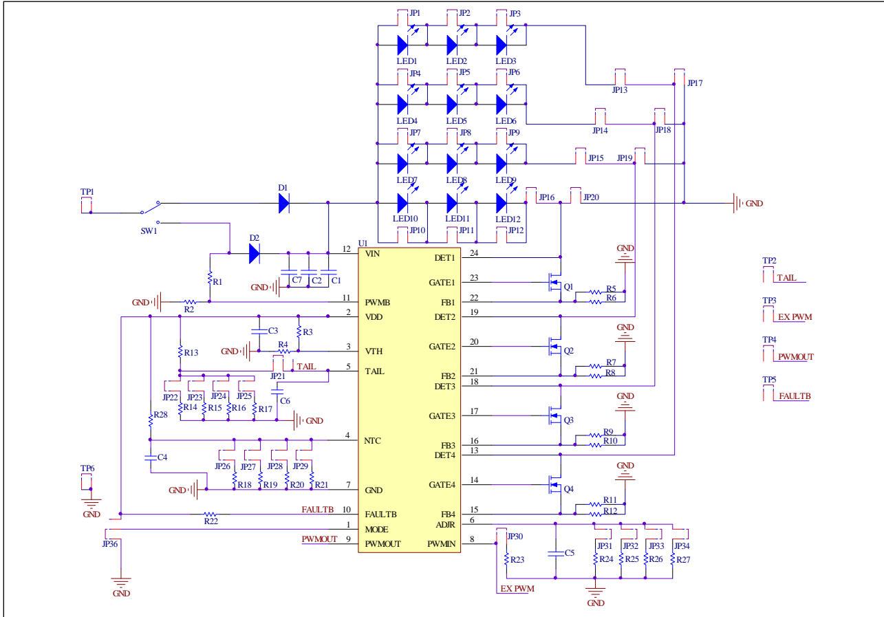
Figure 2: IS32LT3123 Application Schematic
