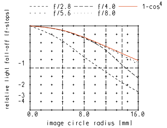
relative light fall-off at ratio 0.05x
