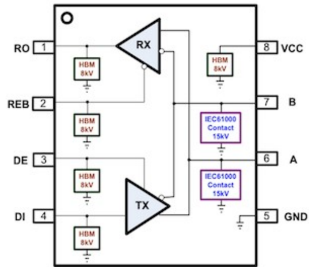
Functional Block of AZRS3078
