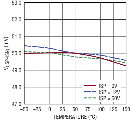
V_{(ISP-ISN)} Regulation vs V_{ISP}
