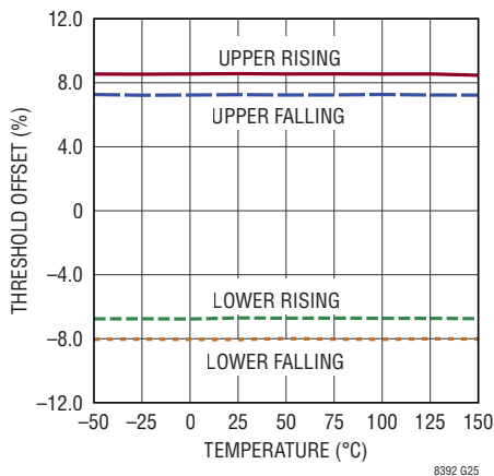
PGOOD Thresholds
