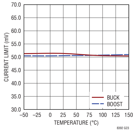
Maximum Current Sense vs Temperature
