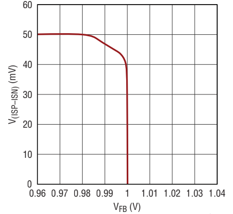
V_{(ISP-ISN)} Regulation vs V_{FB}
