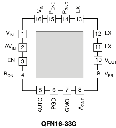
Fig. 3 - SiP12107 Pin Configuration (Top View)
