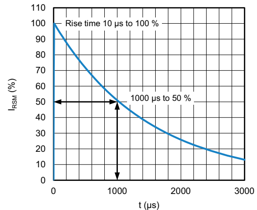
Fig. 3 - 10/10 000 \mu\text{s} Peak Pulse Current Wave Form
