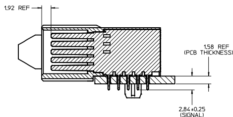
SECTION Z-Z
