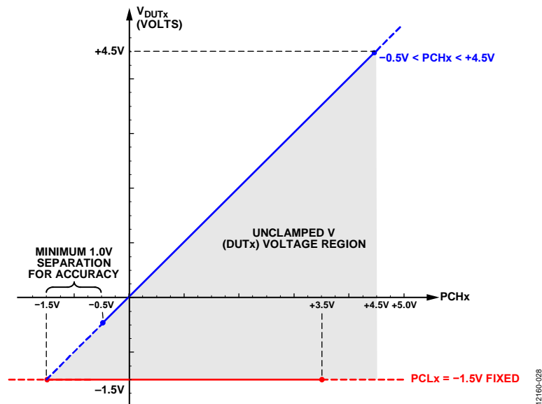
Figure 131. PPMU Voltage Clamp High, Functional Diagram (Voltage Clamp Low Fixed at -1.5 V)
