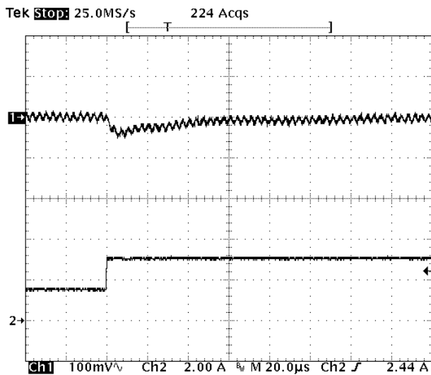
Fig-2.5V-6: Output voltage response for V_{out}=2.5V to positive load current step-change from 1.5A to 3A with slew rate of 3A/\mu s at V_{in}=5.0V . C_o=47\mu F \times 2 ceramic.
