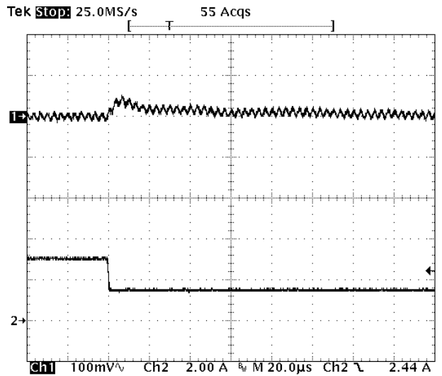
Fig-2.5V-7: Output voltage response for V_{out}=2.5V to positive load current step-change from 3A to 1.5A with slew rate of -5A/\mu s at V_{in}=5.0V . C_o=47\mu F \times 2 ceramic.
