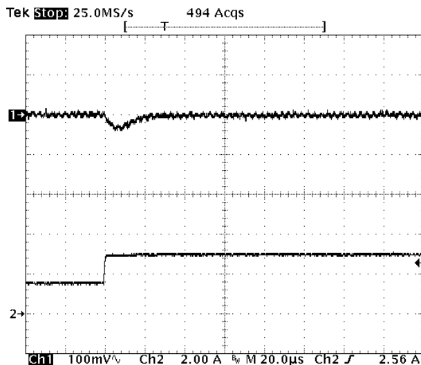
Fig-0.7525V-6: Output voltage response for V_{out}=0.7525V to positive load current step-change from 1.5A to 3A with slew rate of 3A/\mu s at V_{in}=5.0V . C_o=47\mu F \times 2 ceramic.
