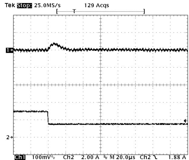
Fig-0.7525V-7: Output voltage response for V_{out}=0.7525V to positive load current step-change from 3A to 1.5A with slew rate of -5A/\mu s at V_{in}=5.0V . C_o=47\mu F \times 2 ceramic.
