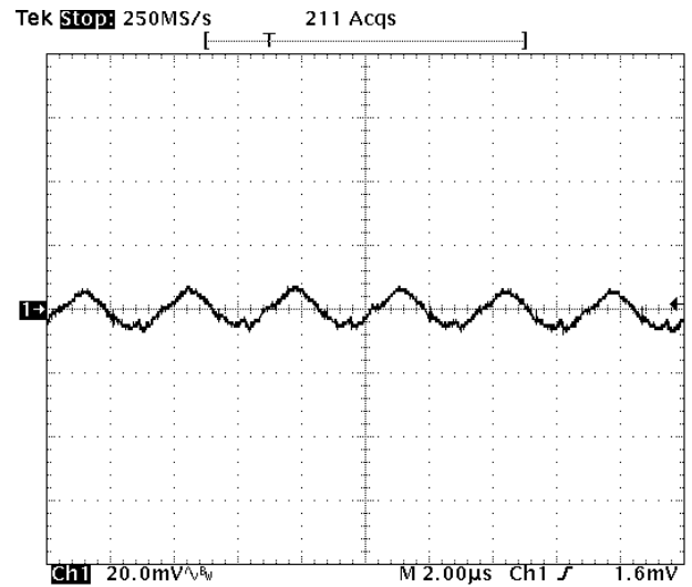
Fig-1.0V-5: Output voltage ripple (20mV/div.) for V_{out}=1.0V at full rated load current into a resistive load with external capacitance 47\mu F \times 2 ceramic + 1\mu F ceramic at V_{in}=5.0V . Time scale: 2μs/div
