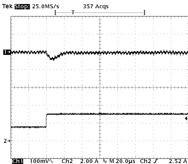
Fig-1.0V-6: Output voltage response for V_{out}=1.0V to positive load current step-change from 1.5A to 3A with slew rate of 3A/\mu s at V_{in}=5.0V . C_o=47\mu F \times 2 ceramic. Top trace: output voltage (100mV/div.) Bottom trace: load current (2A/div.) Time scale: 20μs/div.
