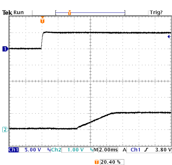
Fig-1.0V-4: Turn-on transient for V_{out}=1.0V with application of V_{in} at full rated load current (resistive) and 47\mu F \times 2 external capacitance at V_{in}=5.0V . Top trace: V_{in} (5V/div.) Bottom trace: output voltage (1V/div.) Time scale: 2ms/div.
