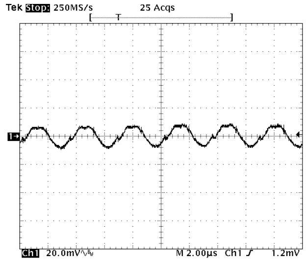
Fig-2.5V-5: Output voltage ripple (20mV/div.) for V_{out}=2.5V at full rated load current into a resistive load with external capacitance 47\mu F \times 2 ceramic + 1\mu F ceramic at V_{in}=5.0V .
