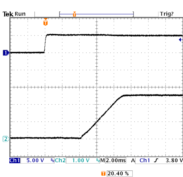
Fig-2.5V-4: Turn-on transient for V_{out}=2.5V with application of V_{in} at full rated load current (resistive) and 47\mu F \times 2 external capacitance at V_{in}=5.0V .
